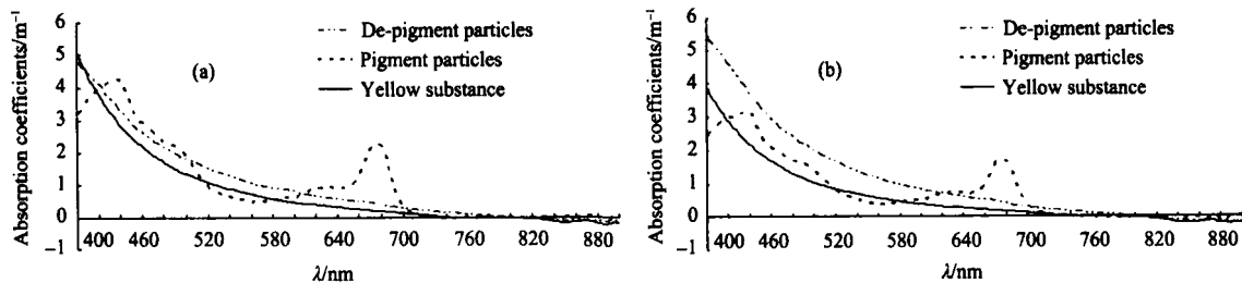
Fig. 2 Natural water absorption spectral curves of three-component in the experiment fields
